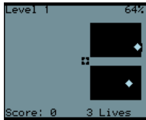
Figure 10.27.: Xbox
