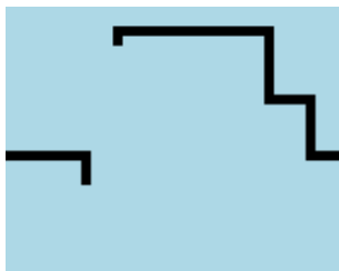
Figure 10.19.: Snake
