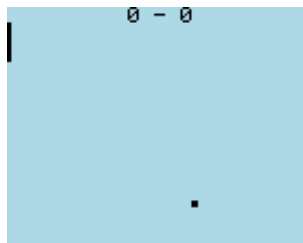
Figure 10.15.: Pong
