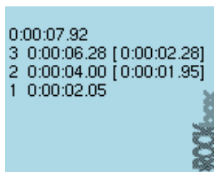
Figure 10.50.: Stopwatch
