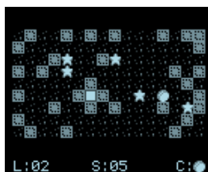
Figure 10.24.: Star game
