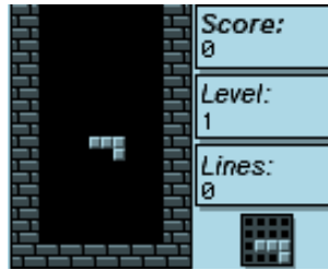
Figure 10.17.: Rockblox
