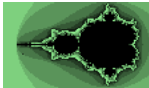
Figure 11.30.: Fractals: Mandelbrot set
