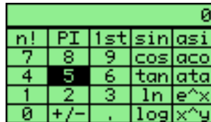
Figure 11.43.: Calculator
