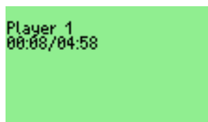
Figure 11.45.: Chess Clock
