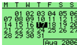
Figure 11.44.: Calendar
