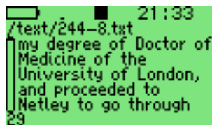
Figure 11.39.: Text Viewer
