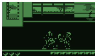
Figure 11.42.: ZXBox
