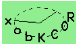
Figure 11.26.: Bounce
