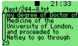
Figure 11.41.: A bookmark
