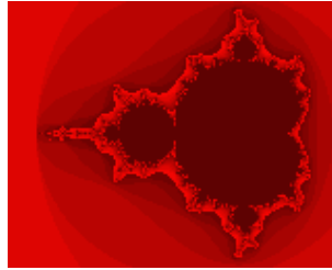
Figure 10.31.: Fractals: Mandelbrot set
