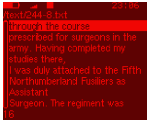
Figure 10.41.: A bookmark
