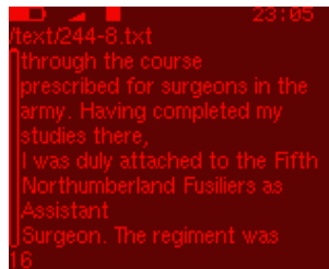
Figure 10.39.: Text Viewer
