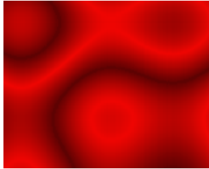
Figure 10.35.: Plasma
