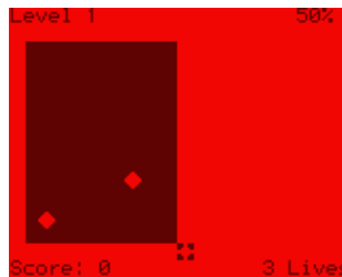
Figure 10.26.: Xbox
