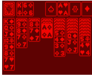
Figure 10.21.: Klondike solitaire
