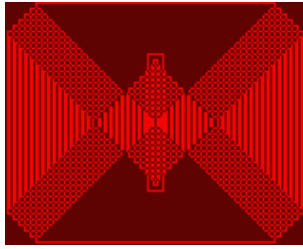
Figure 10.32.: Mosaïque
