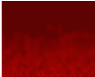
Figure 10.30.: Fire
