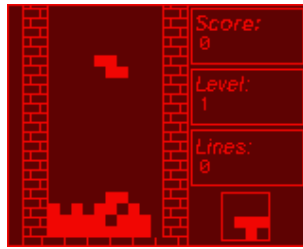
Figure 10.16.: Rockblox
