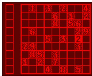
Figure 10.24.: Sudoku
