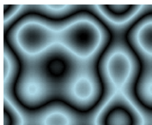
Figure 10.36.: Plasma
