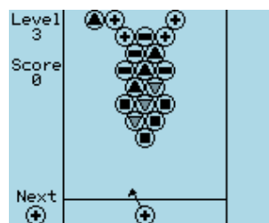
Figure 10.3.: Bubbles
