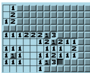
Figure 10.13.: Minesweeper plugin
