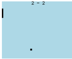
Figure 10.15.: Pong
