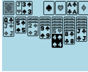
Figure 10.22.: Klondike solitaire
