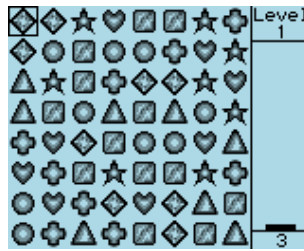
Figure 10.11.: Jewels
