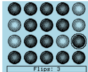
Figure 10.7.: Flipit
