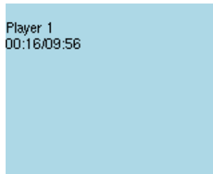
Figure 10.45.: Chess Clock
