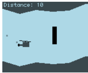
Figure 10.5.: Chopper
