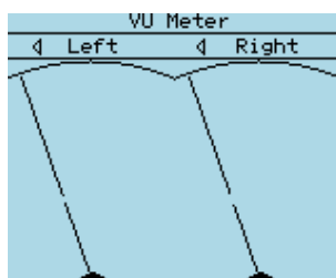
Figure 10.39.: VU-Meter
