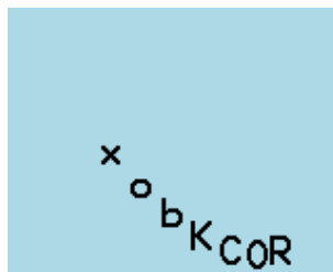
Figure 10.28.: Bounce
