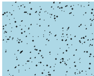
Figure 10.38.: Starfield
