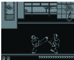
Figure 10.43.: ZXBox
