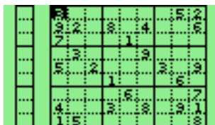
Figure 11.23.: Sudoku
