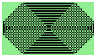
Figure 11.31.: Mosaique
