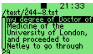
Figure 11.40.: A bookmark
