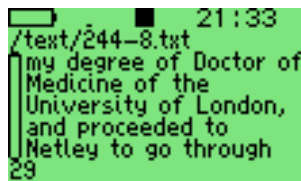
Figure 11.38.: Text Viewer
