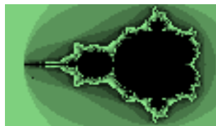
Figure 11.30.: Fractals: Mandelbrot set
