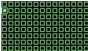
Figure 10.11.: Minesweeper plugin
