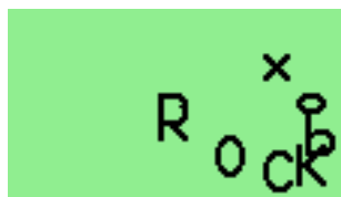
Figure 11.26.: Bounce
