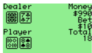
Figure 11.1.: Blackjack
