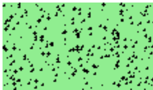
Figure 11.36.: Starfield
