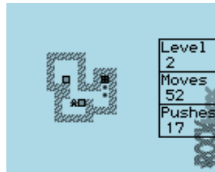
Figure 10.21: Sokoban
