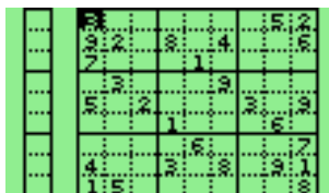
Figure 11.23: Sudoku
