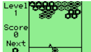
Figure 11.3: Bubbles
