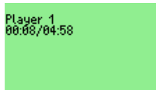
Figure 11.44: Chess Clock
