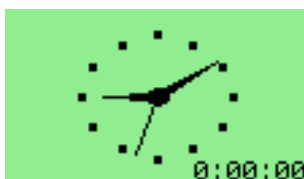
Figure 11.45: Clock
