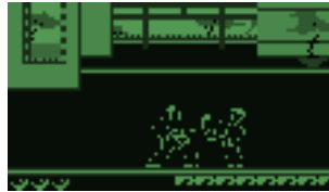
Figure 11.41: ZXBox
