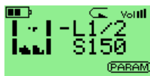
Figure 10.3: Rockblox
