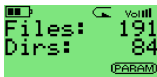
Figure 10.11: The stats-plugin
