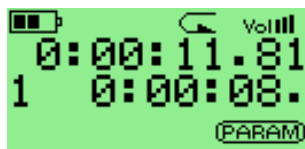
Figure 10.12: Stopwatch
