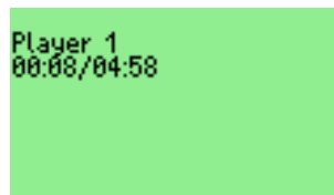
Figure 10.44: Chess Clock
