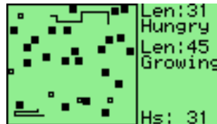
Figure 10.24: Wormlet game
