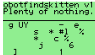
Figure 11.14: Robotfindskitten
