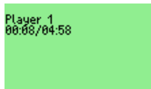
Figure 11.44: Chess Clock
