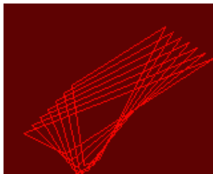
Figure 10.29: Demystify
