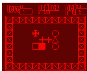
Figure 10.13: pegbox
