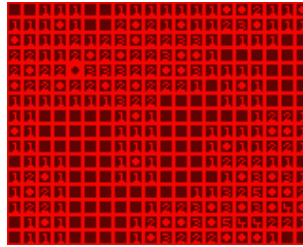
Figure 10.12: Minesweeper plugin
