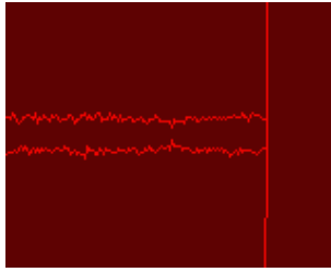
Figure 10.33: Oscilloscope
