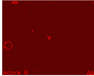
Figure 10.22: Spacerocks
