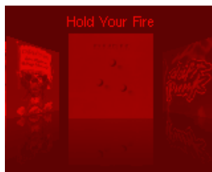
Figure 10.34: PictureFlow
