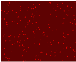
Figure 10.37: Starfield
