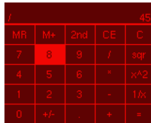
Figure 10.40: Calculator
