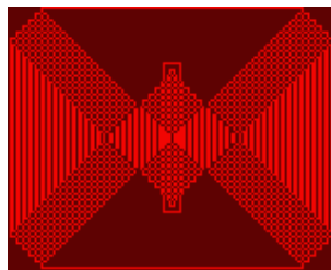
Figure 10.32: Mosaique
