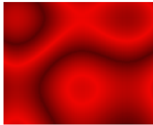
Figure 10.35: Plasma
