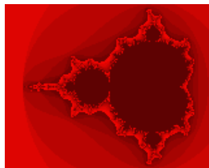
Figure 10.31: Mandelbrot
