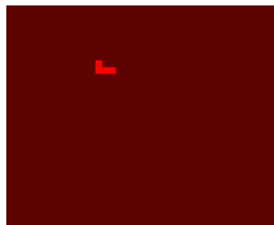
Figure 10.18: Snake
