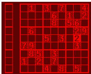
Figure 10.24: Sudoku
