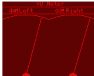
Figure 10.38: VU-Meter
