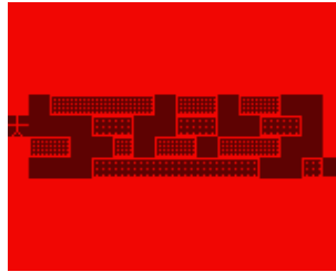
Figure 10.11: MazezaM
