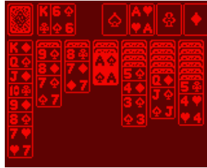
Figure 10.21: Klondike solitaire
