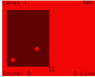
Figure 10.26: Xbox
