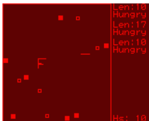
Figure 10.25: Wormlet game
