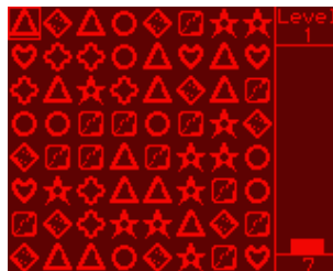
Figure 10.10: Jewels
