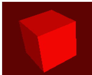
Figure 10.28: Cube
