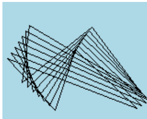
Figure 11.30: Demystify
