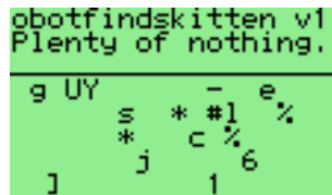
Figure 10.14: Robotfindskitten
