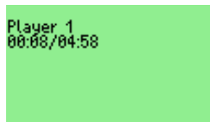
Figure 10.41: Chess Clock
