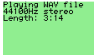
Figure 10.38: Wavplay
