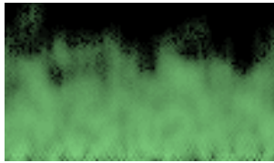
Figure 10.29: Fire
