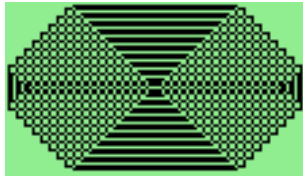
Figure 11.31: Mosaïque
