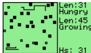
Figure 11.24: Wormlet game
