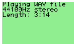
Figure 11.38: Wavplay
