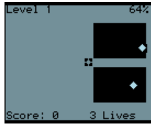
Figure 10.26: Xobox
