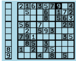
Figure 10.24: Sudoku
