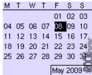
Figure 10.41: Calendar
