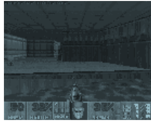
Figure 10.6: Doom
