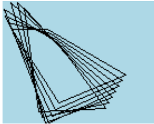
Figure 10.29: Demystify
