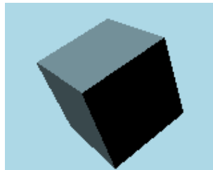
Figure 11.30: Cube
