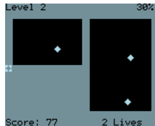
Figure 11.28: Xobox
