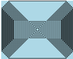
Figure 11.34: Mosaïque
