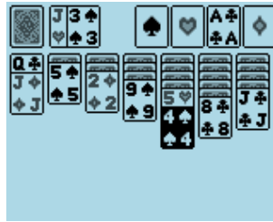
Figure 11.23: Klondike solitaire
