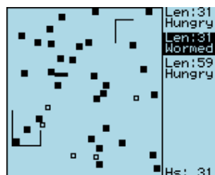
Figure 11.27: Wormlet game
