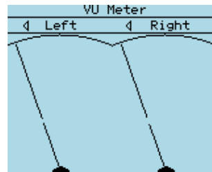
Figure 11.40: VU-Meter
