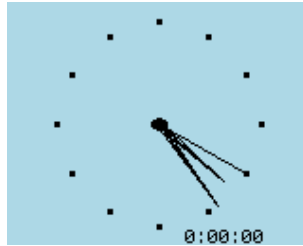
Figure 11.46: Clock
