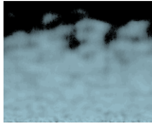
Figure 11.32: Fire
