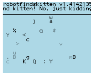
Figure 11.17: Robotfindskitten
