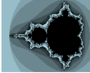
Figure 11.33: Mandelbrot
