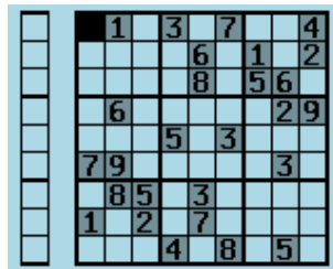
Figure 11.26: Sudoku
