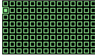
Figure 11.11: Minesweeper plugin
