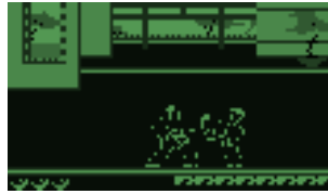
Figure 11.40: ZXBox
