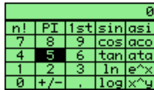
Figure 11.41: Calculator
