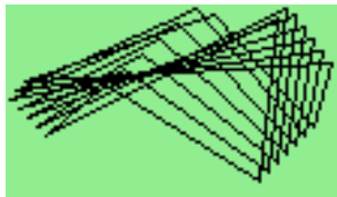
Figure 11.28: Demystify
