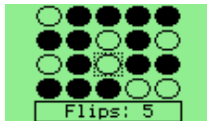
Figure 11.6: Flipit
