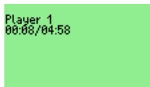
Figure 11.43: Chess Clock
