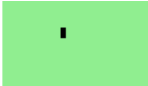
Figure 11.17: Snake
