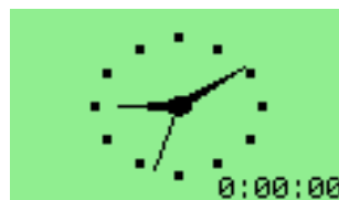
Figure 11.44: Clock
