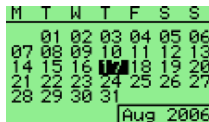
Figure 11.42: Calendar
