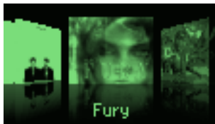
Figure 11.32: PictureFlow
