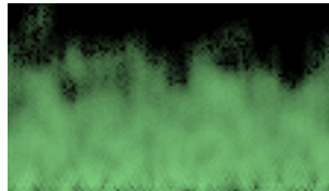
Figure 11.28: Fire
