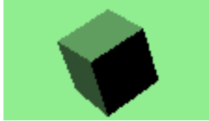
Figure 11.26: Cube
