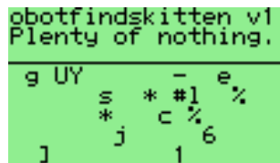
Figure 11.13: Robotfindskitten
