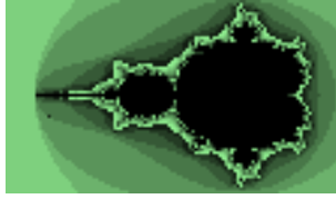
Figure 11.29: Mandelbrot
