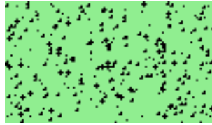
Figure 11.35: Starfield
