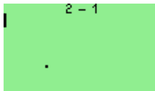
Figure 11.12: Pong
