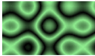
Figure 11.33: Plasma
