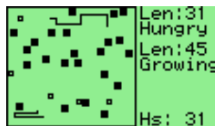
Figure 11.23: Wormlet game
