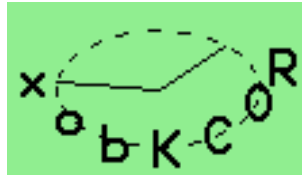
Figure 11.25: Bounce
