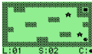
Figure 11.21: Star game
