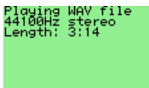
Figure 11.37: Wavplay
