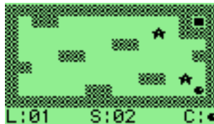
Figure 11.21: Star game
