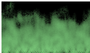
Figure 11.28: Fire
