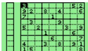
Figure 11.22: Sudoku
