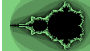
Figure 11.29: Mandelbrot
