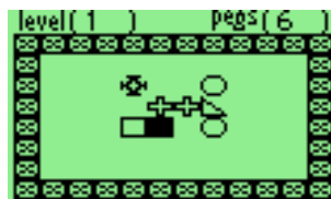
Figure 11.11: pegbox
