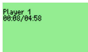
Figure 11.40: Chess Clock
