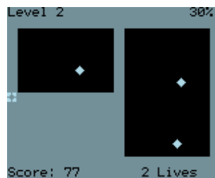
Figure 10.26: Xbox
