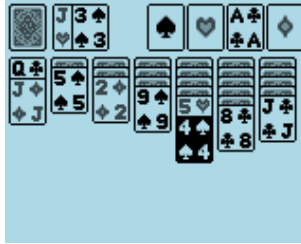
Figure 10.21: Klondike solitaire
