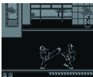
Figure 10.39: ZXBox
