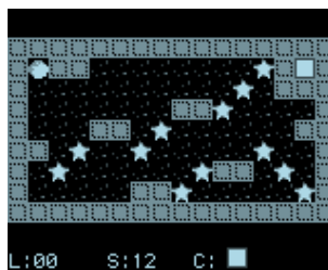
Figure 10.23: Star game
