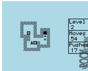
Figure 10.20: Sokoban
