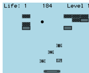
Figure 10.2: BrickMania
