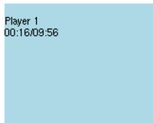
Figure 11.44: Chess Clock
