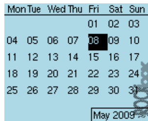
Figure 11.43: Calendar
