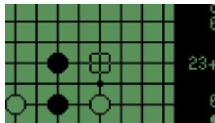
Figure 10.6: Goban
