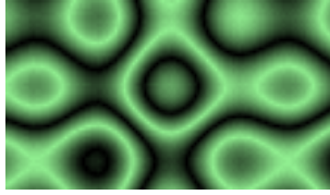
Figure 10.32: Plasma
