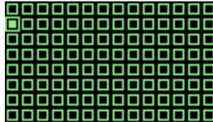
Figure 10.9: Minesweeper plugin
