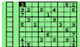
Figure 10.21: Sudoku
