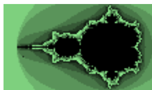
Figure 10.28: Mandelbrot
