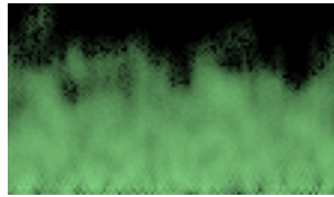
Figure 10.27: Fire
