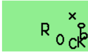
Figure 10.24: Bounce
