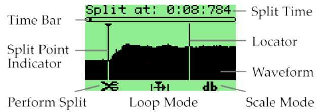
Figure 10.40: The Split Editor’s Main Screen
