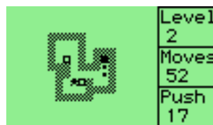
Figure 10.17: Sokoban
