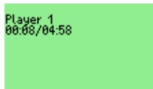
Figure 10.39: Chess Clock
