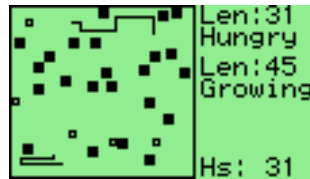
Figure 10.22: Wormlet game
