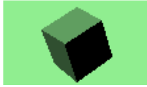
Figure 10.25: Cube
