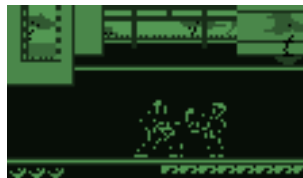
Figure 10.37: ZXBox
