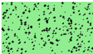
Figure 10.34: Starfield
