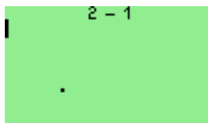
Figure 10.11: Pong
