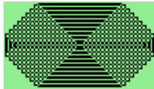
Figure 10.29: Mosaïque
