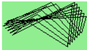
Figure 10.26: Demystify
