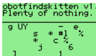
Figure 10.12: Robotfindskitten
