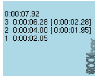
Figure 10.43: Stopwatch
