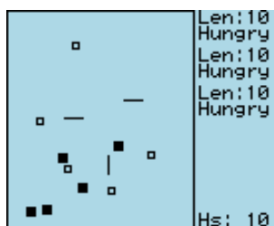
Figure 10.23: Wormlet game
