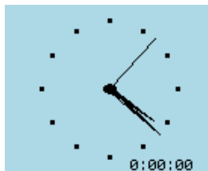
Figure 10.41: Clock
