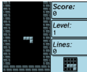
Figure 10.14: Rockblox
