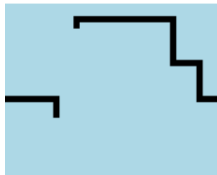
Figure 10.16: Snake
