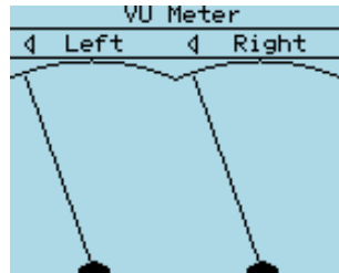
Figure 10.36: VU-Meter
