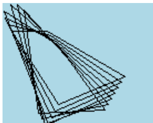
Figure 10.27: Demystify
