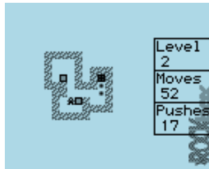
Figure 10.18: Sokoban
