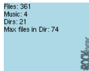
Figure 10.42: The stats-plugin
