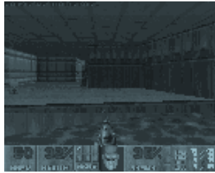
Figure 10.5: Doom
