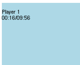
Figure 11.41: Chess Clock
