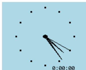
Figure 10.42: Clock
