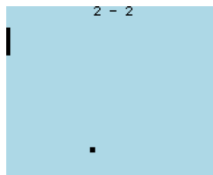
Figure 10.13: Pong
