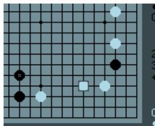
Figure 10.7: Goban
