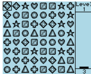
Figure 10.9: Jewels
