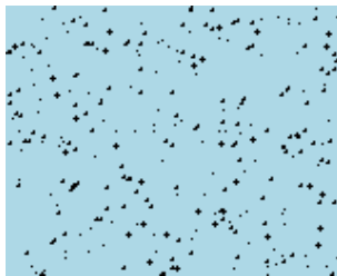
Figure 10.36: Starfield
