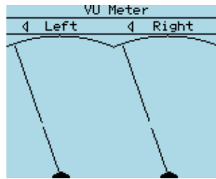
Figure 10.37: VU-Meter
