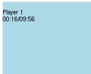
Figure 10.41: Chess Clock
