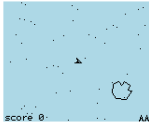
Figure 10.21: Spacerocks
