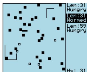
Figure 10.24: Wormlet game
