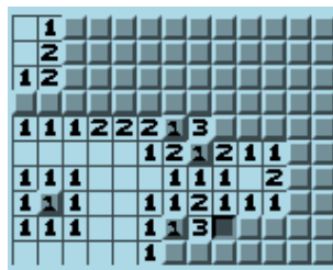
Figure 10.11: Minesweeper plugin
