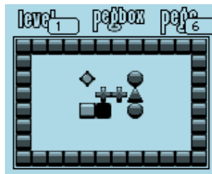
Figure 10.12: pegbox
