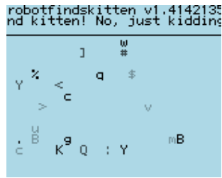
Figure 10.14: Robotfindskitten
