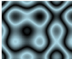
Figure 10.34: Plasma
