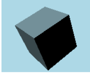
Figure 10.27: Cube
