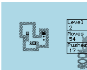
Figure 10.19: Sokoban
