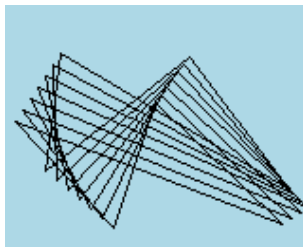
Figure 10.28: Demystify
