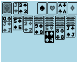
Figure 10.20: Klondike solitaire
