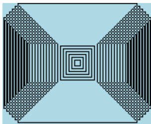
Figure 10.31: Mosaïque
