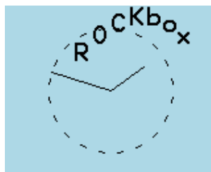
Figure 11.27: Bounce
