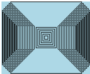
Figure 11.32: Mosaique
