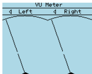
Figure 11.38: VU-Meter
