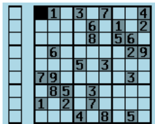
Figure 11.24: Sudoku
