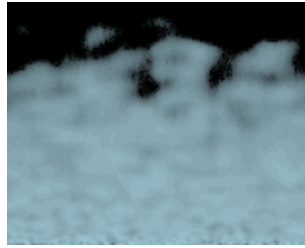
Figure 11.30: Fire
