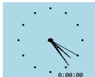
Figure 11.44: Clock
