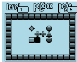
Figure 11.13: pegbox
