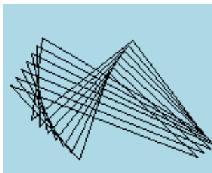
Figure 11.29: Demystify
