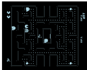
Figure 11.12: Pacbox
