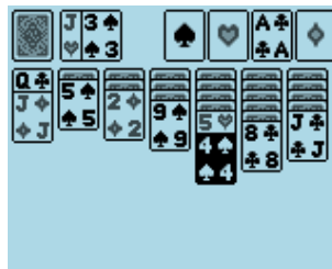
Figure 11.21: Klondike solitaire
