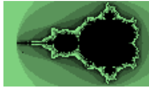
Figure 10.30.: Fractals: Mandelbrot set
