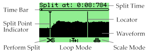
Figure 10.46.: The Split Editor's Main Screen
