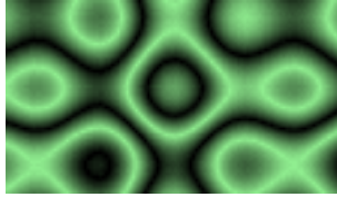
Figure 12.34.: Plasma
