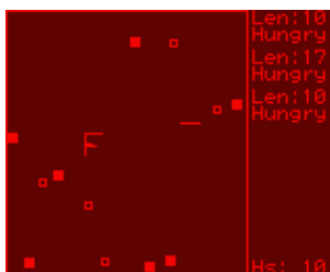
Figure 11.25.: Wormlet game
