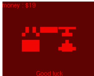
Figure 11.9.: Jackpot
