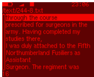
Figure 11.41.: A bookmark
