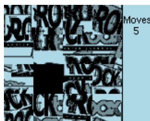
Figure 10.18.: Sliding puzzle
