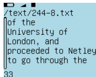
Figure 10.40.: Text Viewer
