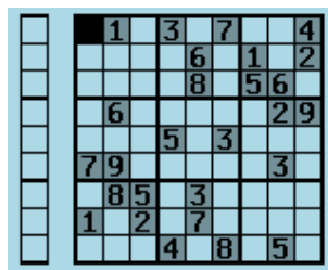
Figure 10.25.: Sudoku
