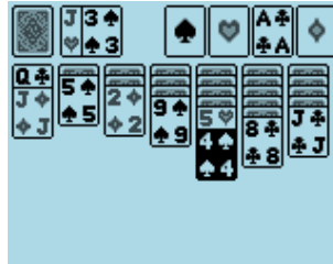
Figure 10.22.: Klondike solitaire
