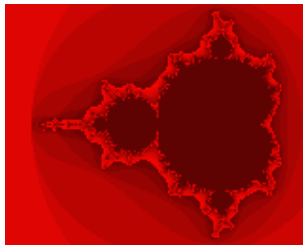
Figure 11.31.: Fractals: Mandelbrot set
