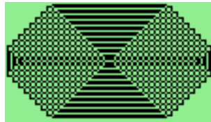
Figure 12.31.: Mosaïque
