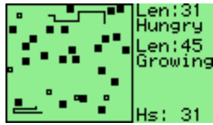
Figure 12.24.: Wormlet game
