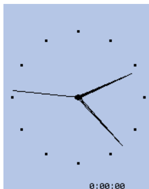
Figure 12.51.: Clock
