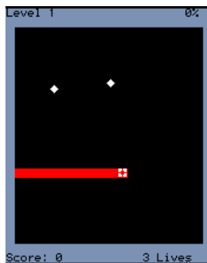
Figure 12.30.: Xbox
