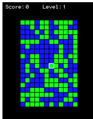
Figure 12.5.: Clix
