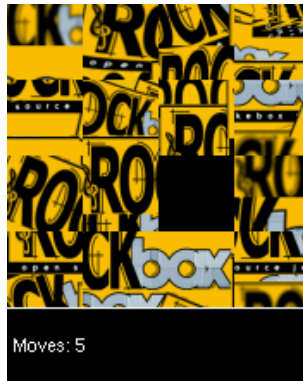
Figure 12.21.: Sliding puzzle
