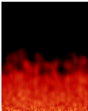
Figure 12.34.: Fire
