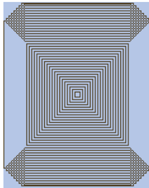
Figure 12.36.: Mosaique
