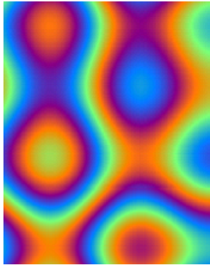
Figure 12.39.: Plasma
