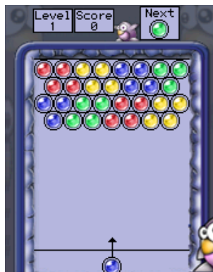
Figure 12.3.: Bubbles
