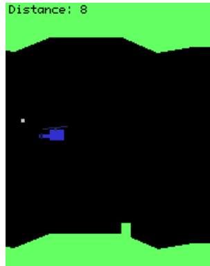
Figure 12.6.: Chopper
