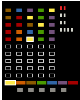
Figure 12.7.: Codebuster
