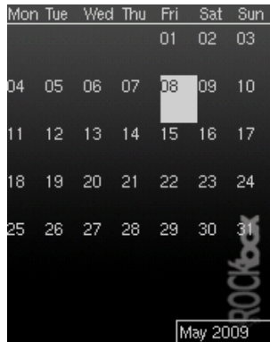
Figure 12.49.: Calendar
