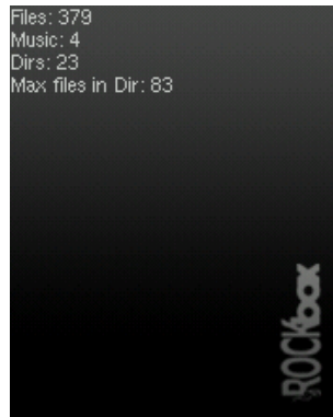
Figure 12.54.: The stats-plugin
