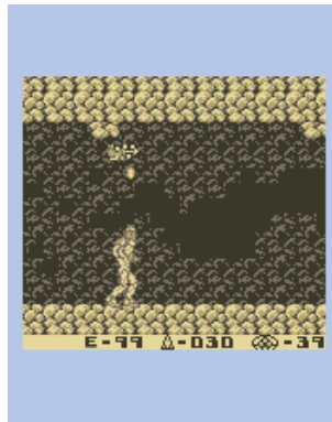
Figure 12.43.: Rockboy
