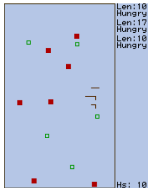
Figure 12.29.: Wormlet game
