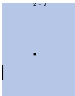
Figure 12.18.: Pong
