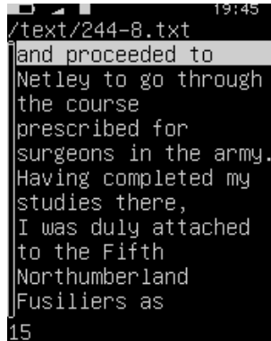
Figure 12.46.: A bookmark
