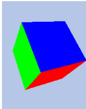
Figure 12.32.: Cube
