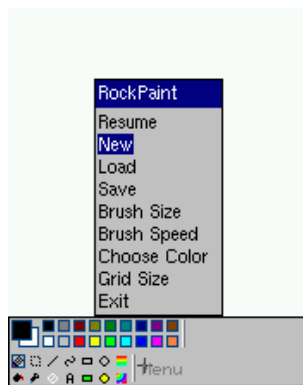
Figure 12.53.: Rockpaint
