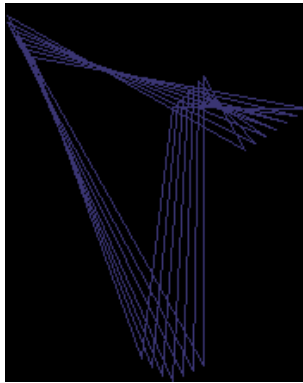
Figure 12.33.: Demystify
