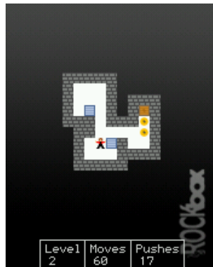
Figure 12.24.: Sokoban
