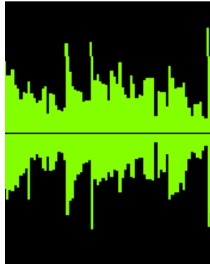
Figure 12.37.: Oscilloscope
