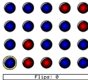
Figure 12.9.: Flipit
