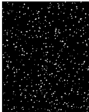
Figure 12.41.: Starfield
