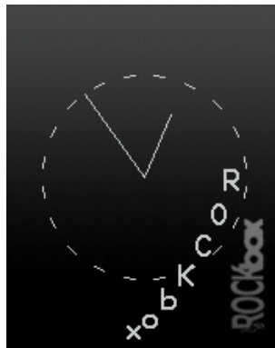
Figure 12.31.: Bounce
