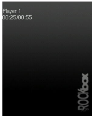
Figure 12.50.: Chess Clock
