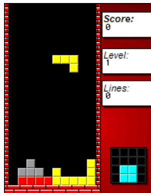
Figure 12.20.: Rockblox
