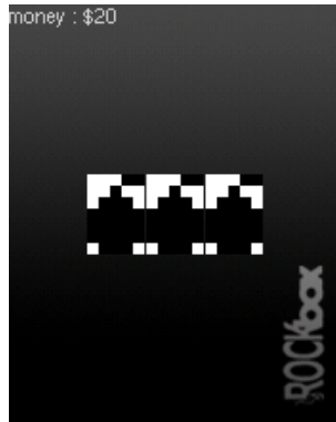
Figure 12.12.: Jackpot
