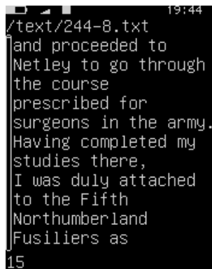
Figure 12.44.: Text Viewer
