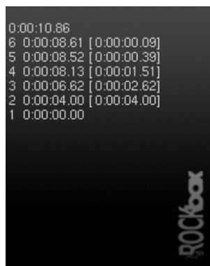
Figure 12.55.: Stopwatch
