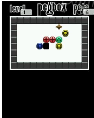
Figure 12.17.: pegbox
