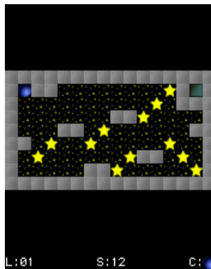
Figure 12.27.: Star game
