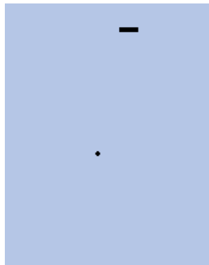
Figure 12.22.: Snake
