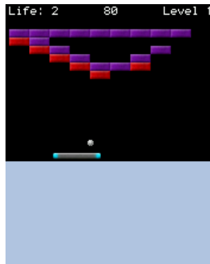
Figure 12.2.: BrickMania
