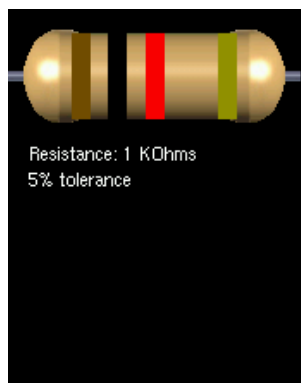
Figure 12.52.: Resistor calculator
