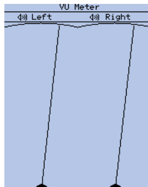
Figure 12.42.: VU-Meter
