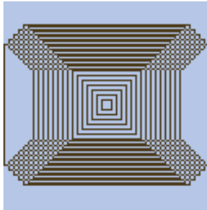
Figure 12.35.: Mosaïque
