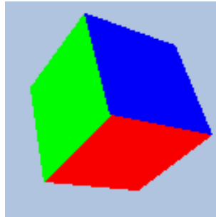
Figure 12.31.: Cube
