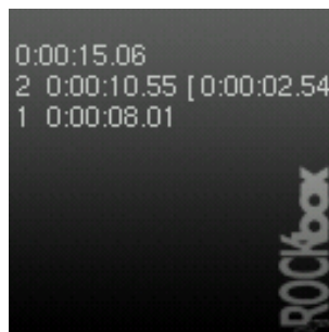
Figure 12.54.: Stopwatch
