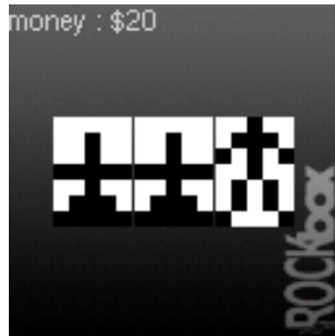
Figure 12.11.: Jackpot
