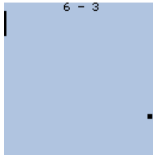
Figure 12.17.: Pong
