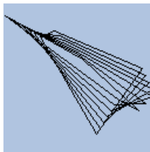
Figure 12.32.: Demystify
