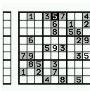
Figure 12.27.: Sudoku
