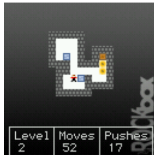
Figure 12.23.: Sokoban
