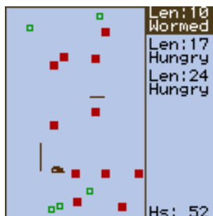
Figure 12.28.: Wormlet game
