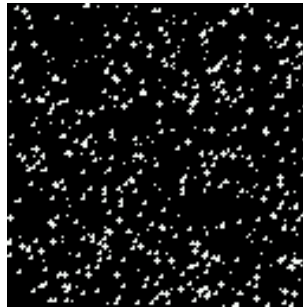
Figure 12.40.: Starfield
