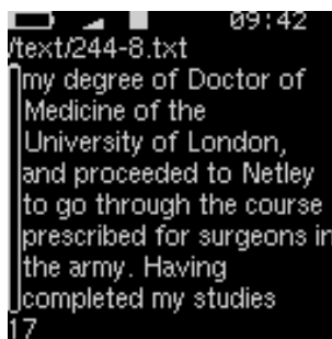
Figure 12.43.: Text Viewer
