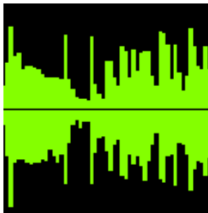
Figure 12.36.: Oscilloscope
