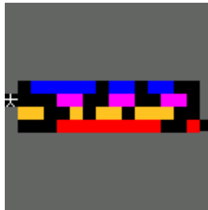
Figure 12.13.: MazezaM
