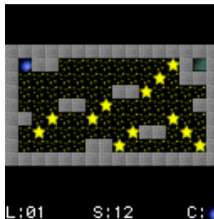
Figure 12.26.: Star game
