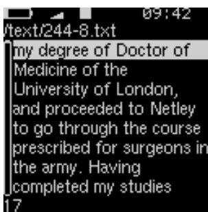
Figure 12.45.: A bookmark
