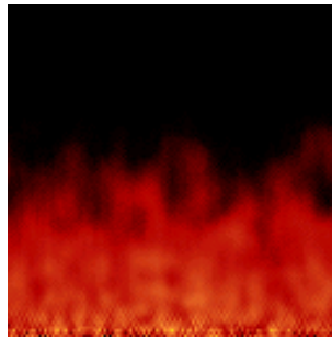
Figure 12.33.: Fire
