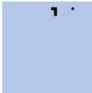
Figure 12.21.: Snake
