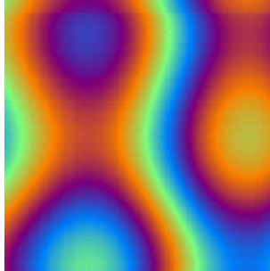
Figure 12.38.: Plasma
