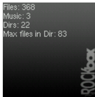
Figure 12.53.: The stats-plugin
