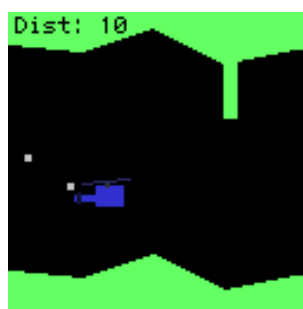
Figure 12.6.: Chopper
