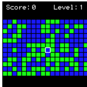
Figure 12.5.: Clix
