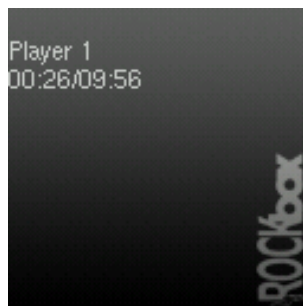
Figure 12.49.: Chess Clock
