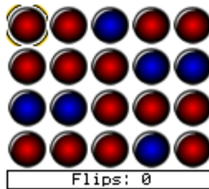
Figure 12.9.: Flipit
