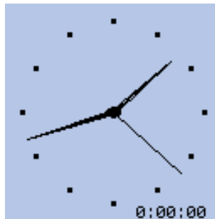
Figure 12.50.: Clock
