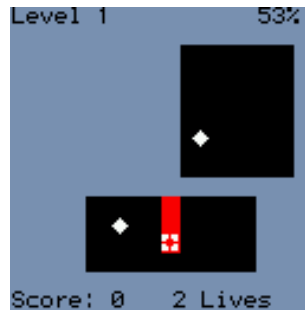
Figure 12.29.: Xbox
