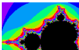
Figure 10.28: Mandelbrot
