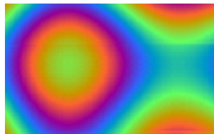
Figure 10.31: Plasma
