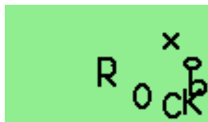
Figure 9.23: Bounce
