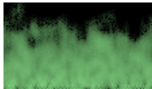
Figure 9.26: Fire
