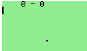
Figure 9.10: Pong
