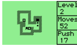
Figure 9.16: Sokoban
