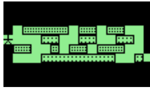
Figure 9.7: MazezaM
