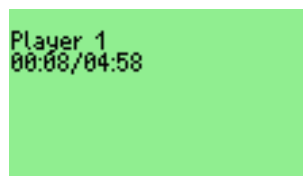
Figure 9.37: Chess Clock
