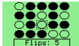
Figure 9.5: Flipit
