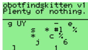
Figure 9.11: Robotfindskitten
