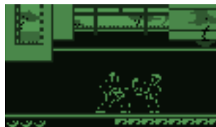
Figure 9.35: ZXBox
