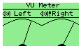
Figure 9.33: VU-Meter
