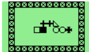
Figure 9.9: pegbox
