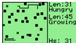
Figure 9.21: Wormlet game
