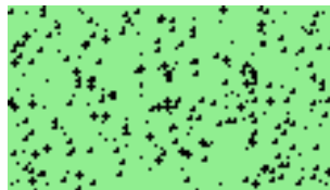
Figure 9.32: Starfield
