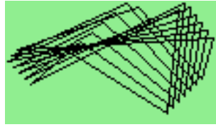
Figure 9.25: Demystify
