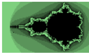
Figure 9.27: Mandelbrot
