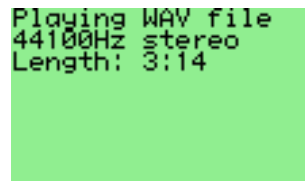
Figure 9.34: Wavplay
