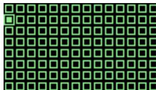
Figure 9.8: Minesweeper plugin
