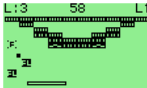
Figure 9.2: BrickMania
