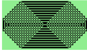
Figure 9.28: Mosaïque
