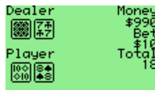
Figure 9.1: Blackjack
