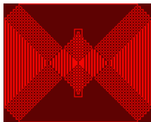
Figure 9.29: Mosaique
