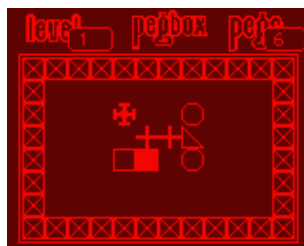
Figure 9.10: pegbox
