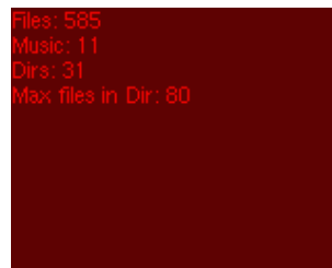
Figure 9.39: The stats-plugin
