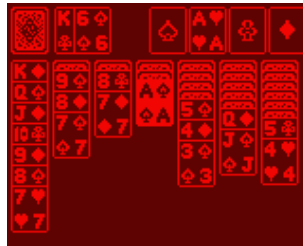
Figure 9.18: Klondike solitaire
