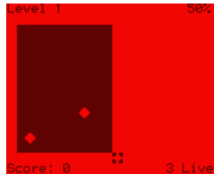
Figure 9.23: Xbox
