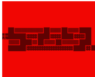
Figure 9.8: MazezaM
