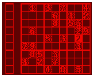
Figure 9.21: Sudoku
