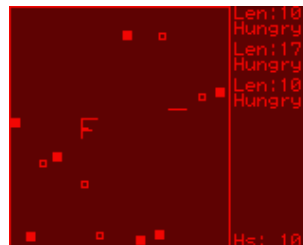
Figure 9.22: Wormlet game
