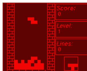
Figure 9.13: Rockblox
