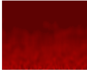
Figure 9.27: Fire
