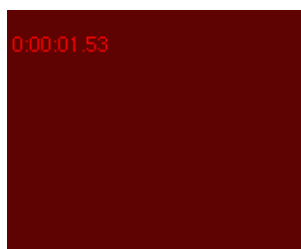
Figure 9.40: Stopwatch
