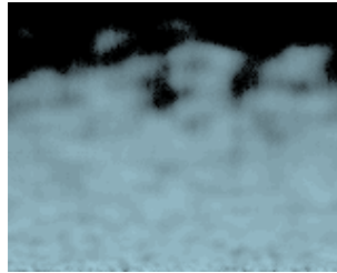
Figure 10.27: Fire
