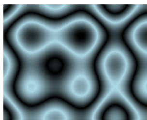
Figure 10.31: Plasma
