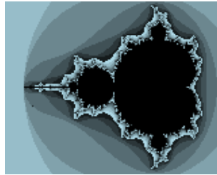
Figure 10.28: Mandelbrot
