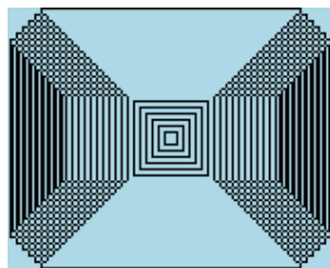
Figure 10.29: Mosaique
