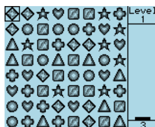
Figure 10.7: Jewels
