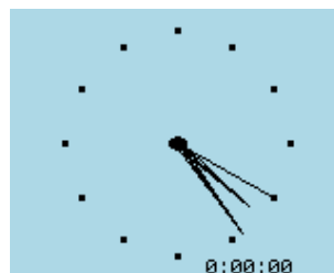
Figure 10.38: Clock
