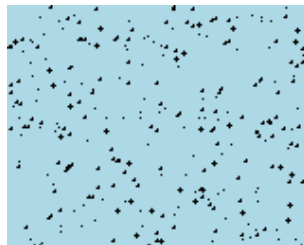
Figure 10.33: Starfield
