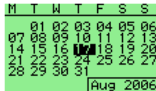
Figure 10.38.: Calendar
