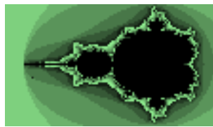
Figure 10.27.: Mandelbrot
