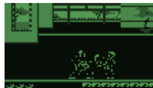
Figure 10.36.: ZXBox
