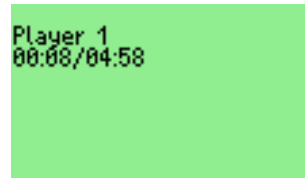
Figure 10.39.: Chess Clock
