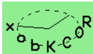
Figure 10.23.: Bounce
