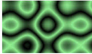
Figure 10.30.: Plasma
