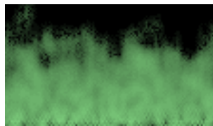
Figure 10.26.: Fire
