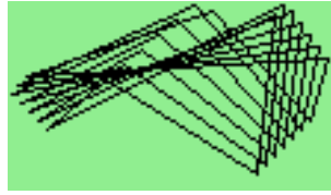
Figure 10.25.: Demystify
