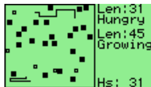
Figure 10.21.: Wormlet game
