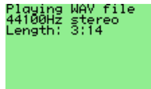
Figure 10.35.: Wavplay
