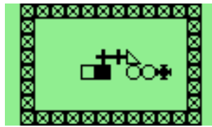
Figure 10.9.: pegbox
