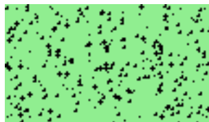
Figure 10.32.: Starfield
