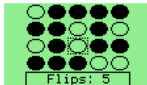
Figure 10.5.: Flipit
