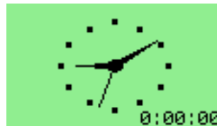
Figure 10.40.: Clock
