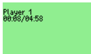
Figure 9.37.: Chess Clock
