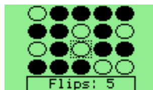
Figure 9.5.: Flipit
