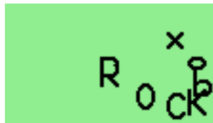
Figure 9.23.: Bounce
