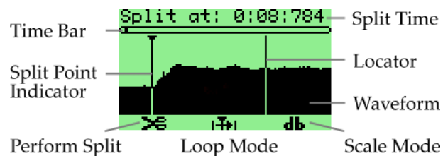
Figure 10.38.: The Split Editor's Main Screen
