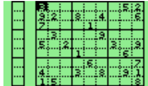
Figure 10.20.: Sudoku
