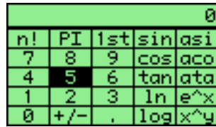
Figure 10.36.: Calculator
