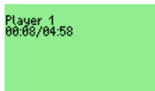
Figure 10.37.: Chess Clock
