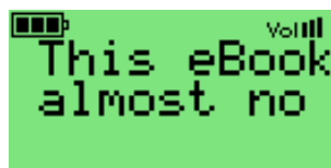
Figure 10.7.: Text Viewer
