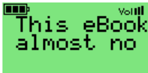
Figure 10.7.: Text Viewer
