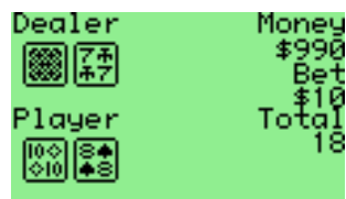
Figure 10.2.: Blackjack
