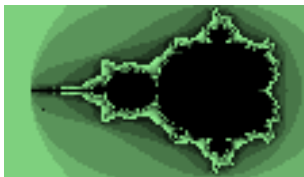
Figure 10.33.: Fractals: Mandelbrot set
